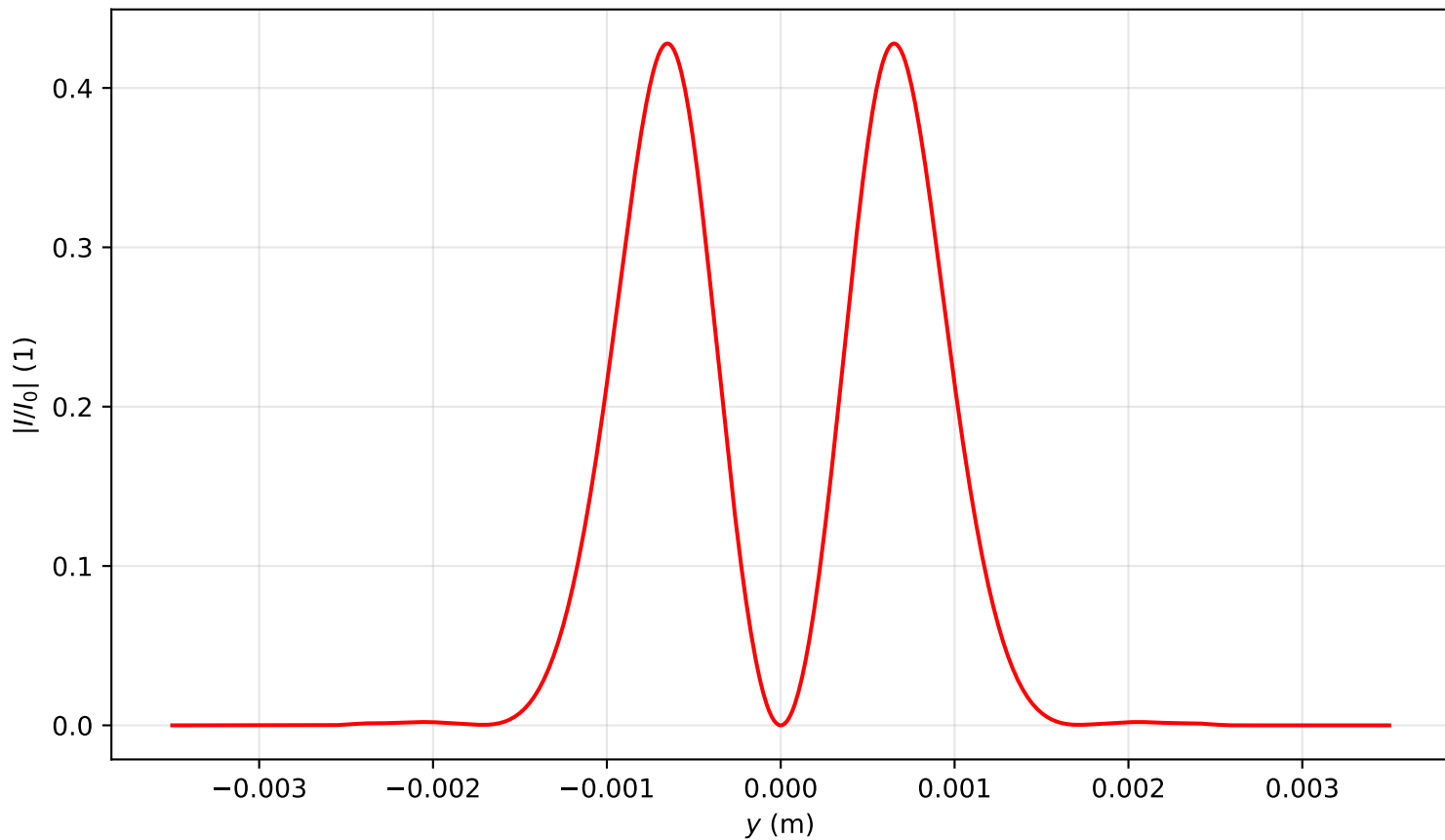
Intensity profile I(x=0, y, z=1.990)/I_0 , P_{in}=3.0P_{cr} , artificial time
